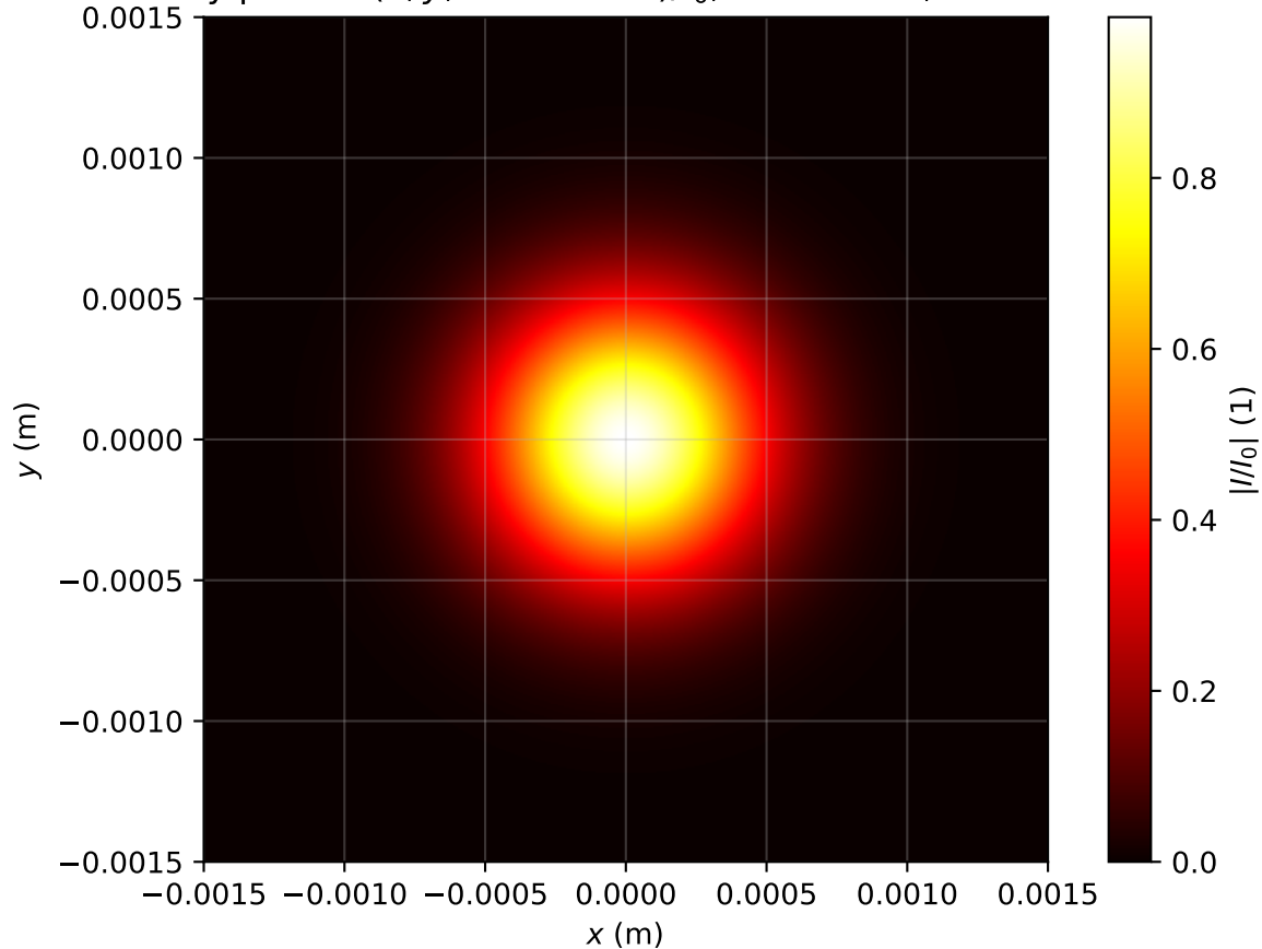
Intensity profile I(x, y, z = 0.398m)/I_0 , P_{in}=0.2P_{cr} , artificial time
